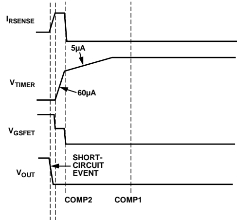
Figure 41. ADM1172-2 Latch Off After Overcurrent Fault
