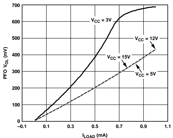
Figure 37. PFO Output Low Voltage vs. Load Current
